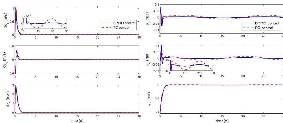
Figure 2. Tracking error of some parameters of the UAV control system
