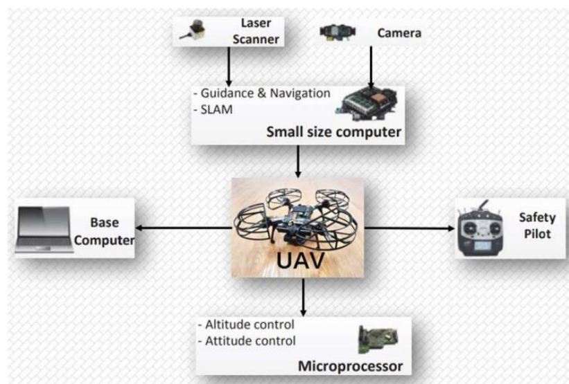
Figure 3. Hardware platform for UAV flight experiment
